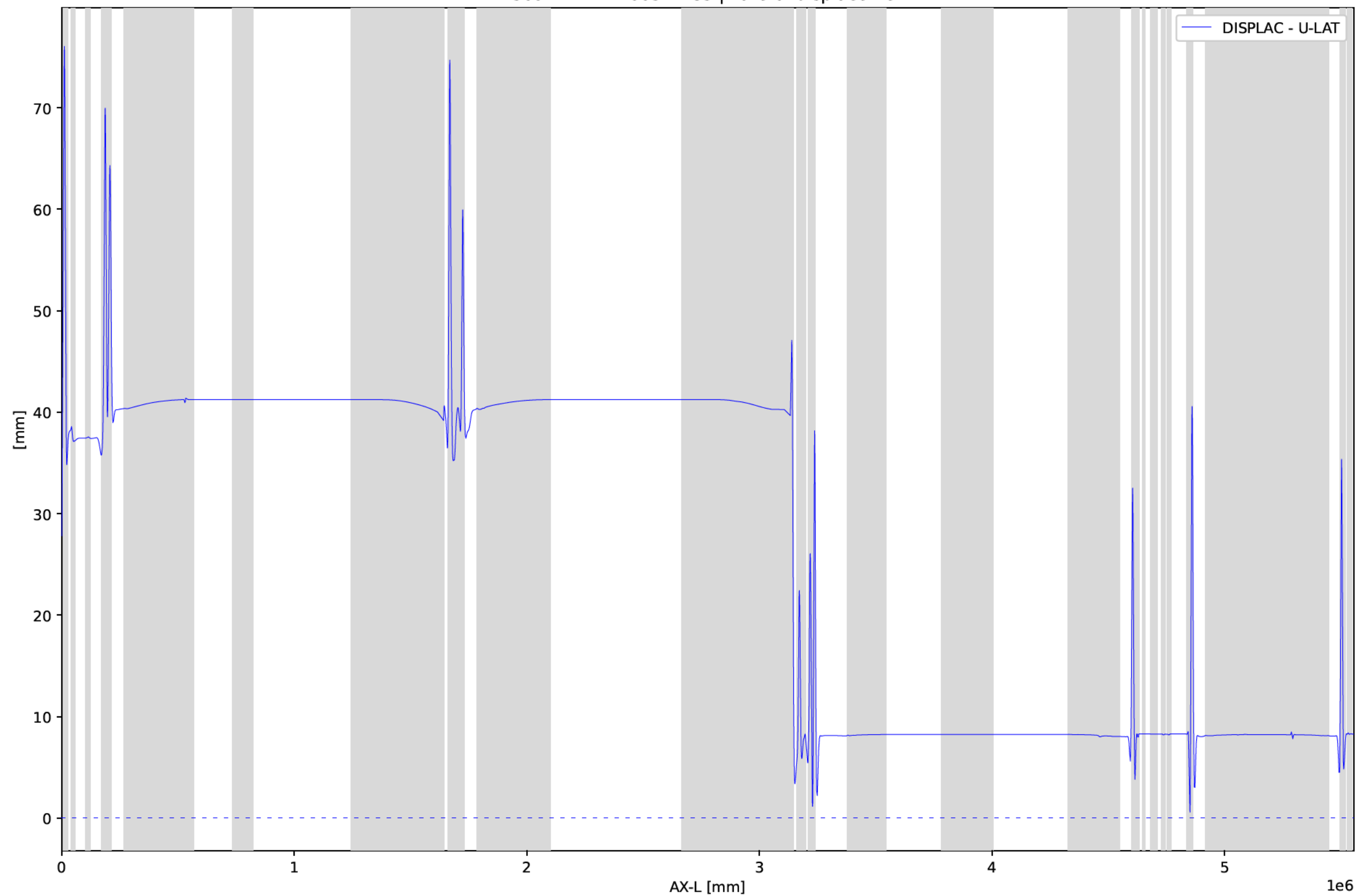
250921 - RA24005 - BC3 | Lateral displacement
