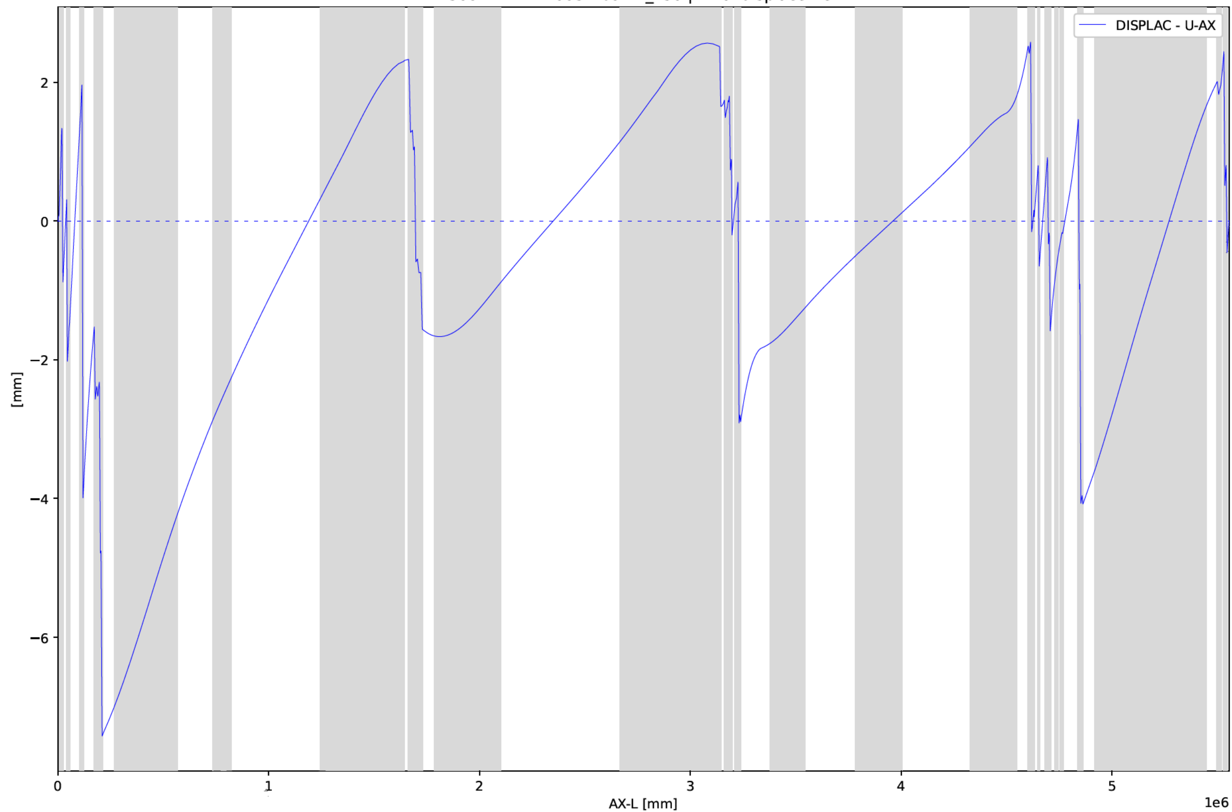
250921 - RA24005 - b01.1_P30 | Axial displacement
