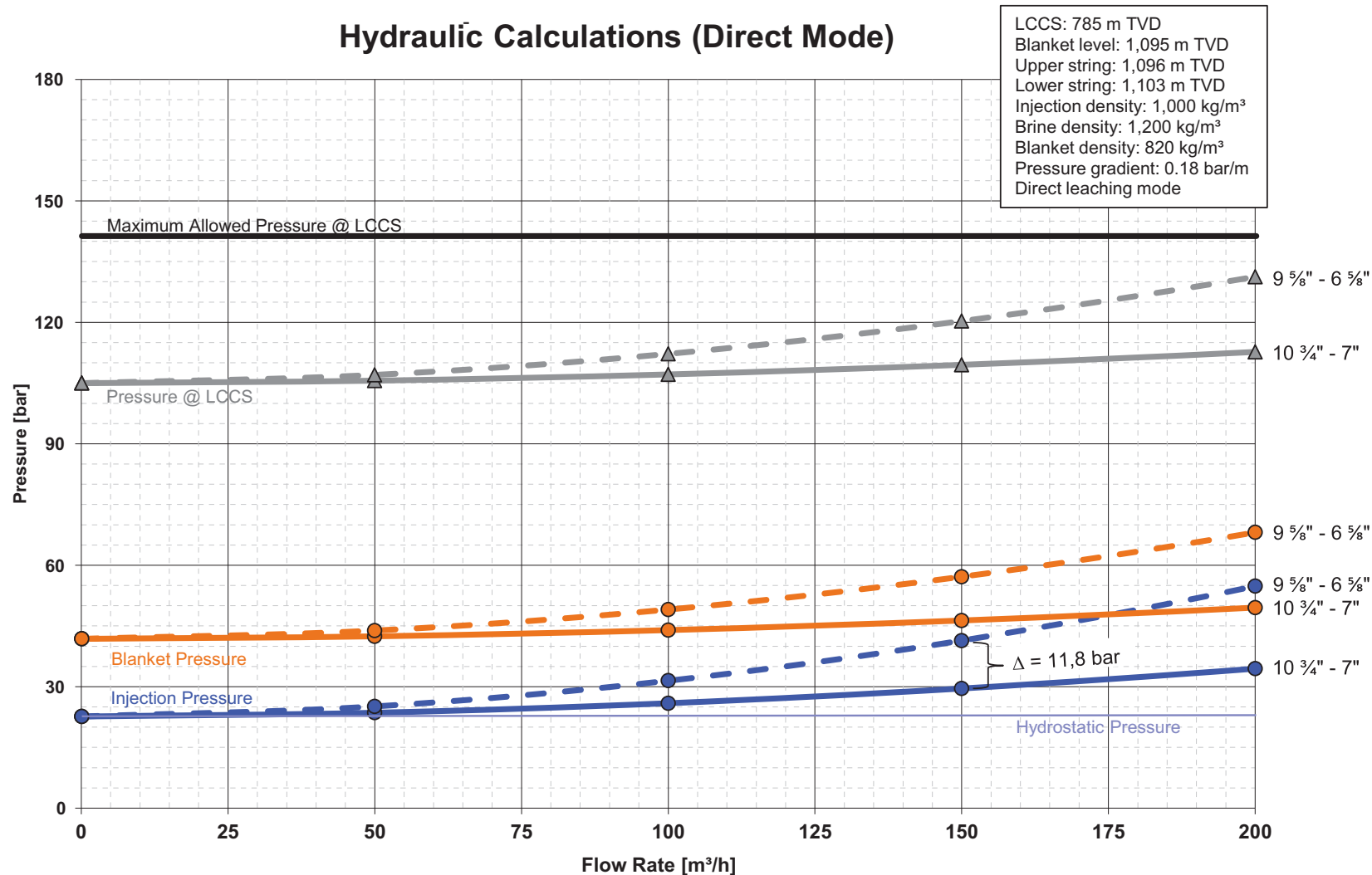
Enclosure 4: Hydraulic calculation for sump leaching phase (direct mode) for 10 3/4" x 7" and 9 5/8" x 6 5/8" leaching combination
