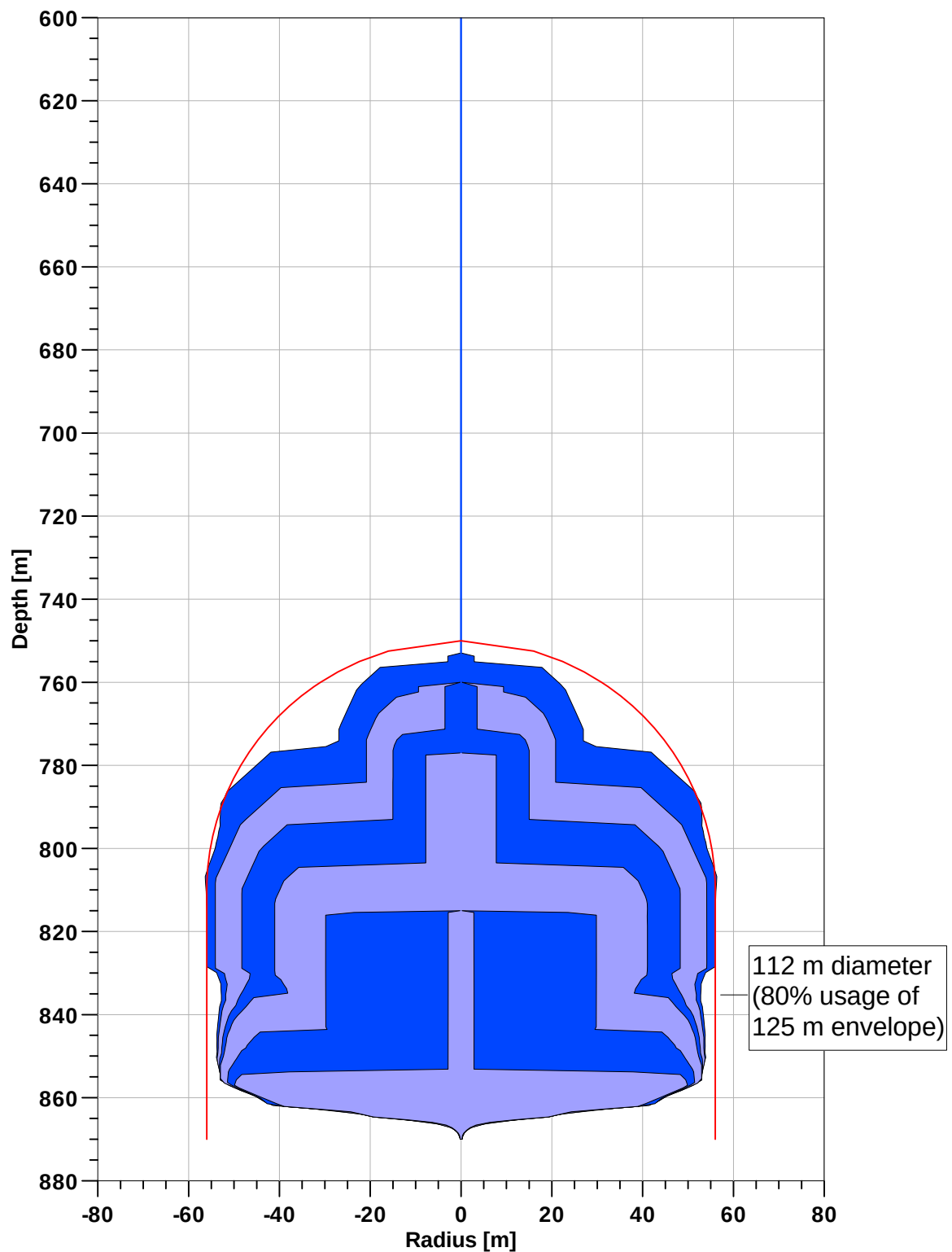
Encl. 12: Type 4, cavern shape development, 20 m cylindrical height.
