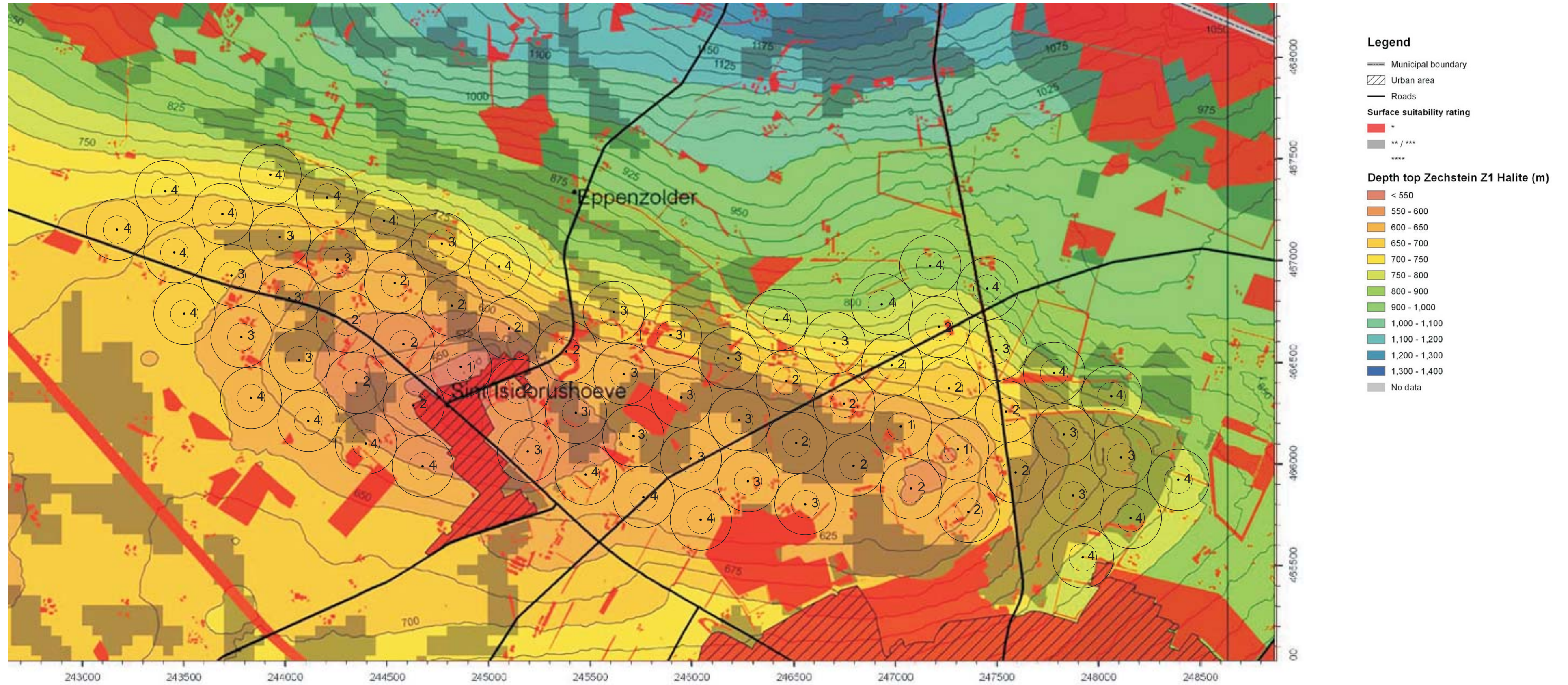
Enclosure 1: Haaksbergen salt pillow, iso-contour map of modelled top Z1 (Werra) Salt (from [1]) and proposed brine production cavern field layout.
