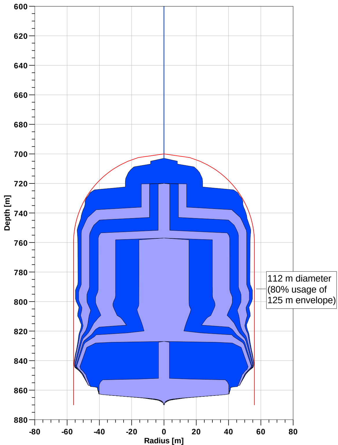
Encl. 5: Type 3, cavern shape development, 70 m cylindrical height (reference cavern).
