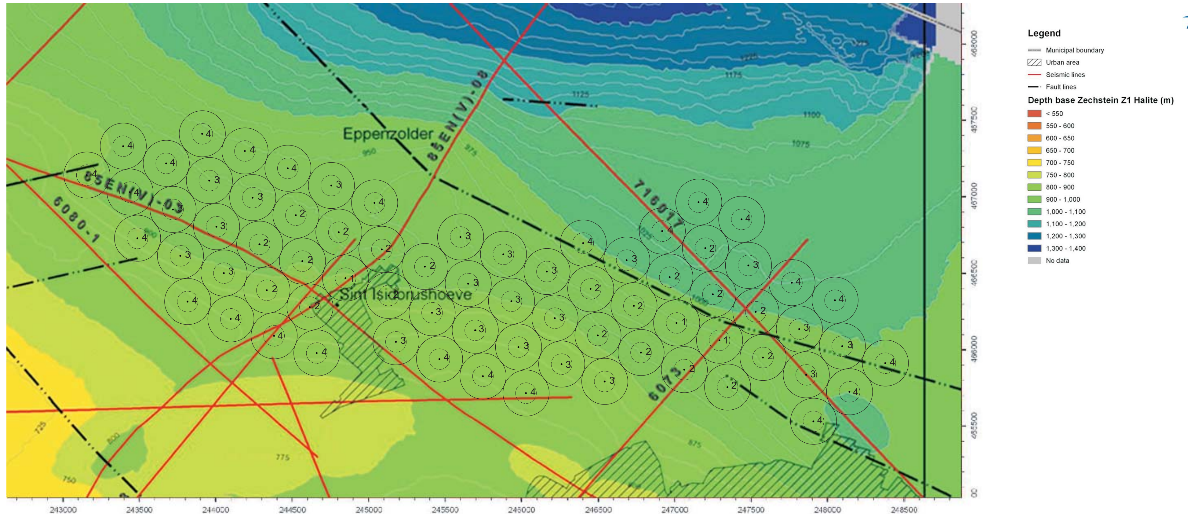
Enclosure 2: Haaksbergen salt pillow, iso-contour map of modelled base Z1 (Werra) Salt (from [1]) and proposed brine production cavern field layout.
