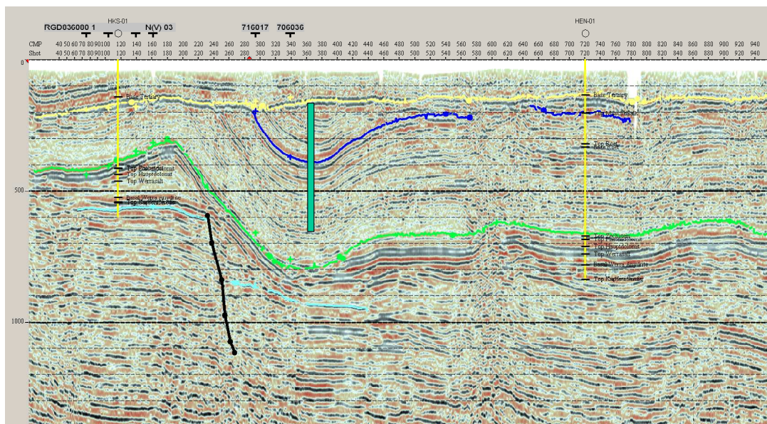
Figure 5.1.1 Regional seismic section through HKS-1 and HEN-1 (both wells are projected onto the line). The green bar shows the minimum amount of removed overburden (uplift) at the culmination of the Haaksbergen salt pillow.
