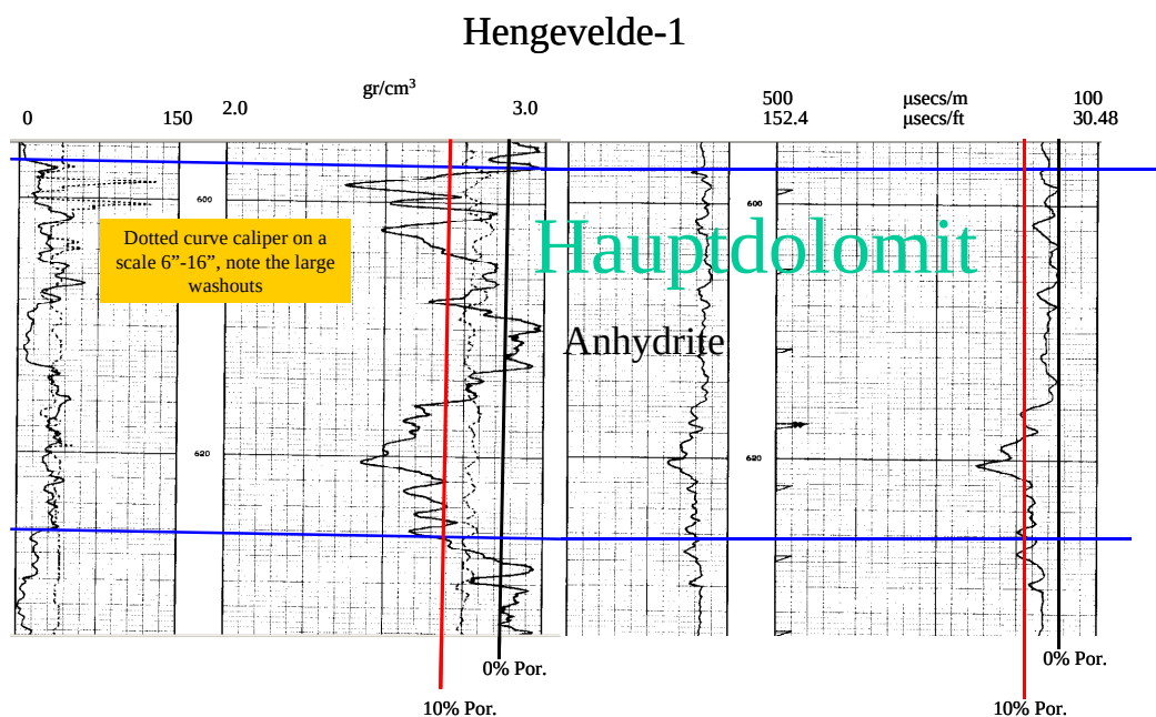
Figure 4.2.5 Log panel across the Hauptdolomit in the well Hengevelde-1. The 0% and 10% porosity values are given based on the assumption that the Hauptdolomit is mainly dolomite ( \text{CaCO}_3 \text{ MgCO}_3 ). The interval is overlain and underlain by anhydrite (high density values). Commonly an anhydrite layer occurs in the middle of the interval. Note that in particular the lower part of the interval shows porosities in excess of 10%. No correction for salinity has been made, consequently the porosity values are slightly too high. The higher porosities in the upper part occur across badly washed out intervals and consequently are suspect. The washouts may, however, be indicative of fractured zones. The washouts may also be indicative of the presence of salt (dissolves in the mud), but the density doesn't support salt (too high).
