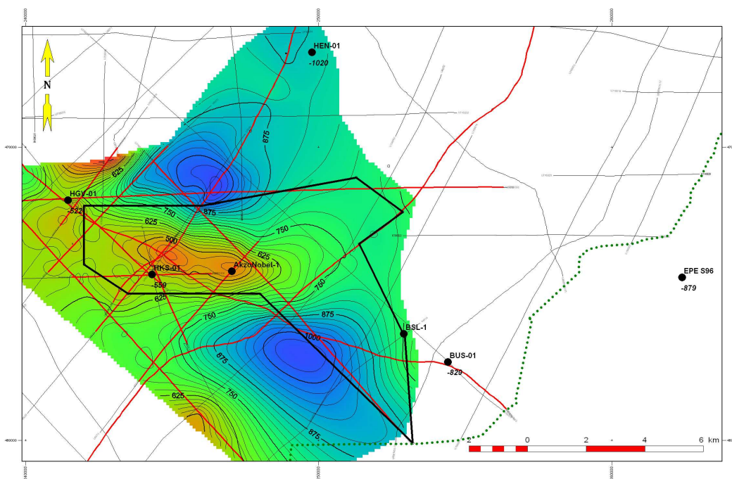
Figure 4.1.3.1 Depth contour map of the top Zechstein. Contour values in m below SRD, contour interval 25 m. The depth conversion is only based on the HKS-1 well and is not appropriate for the area around HEN-1 and BUS-1 (note the differences with the well values, which are plotted next to the well symbols). Note that the HKS-1 well is located slightly above the spill point towards the west. Map is included as Enclosure 2.
