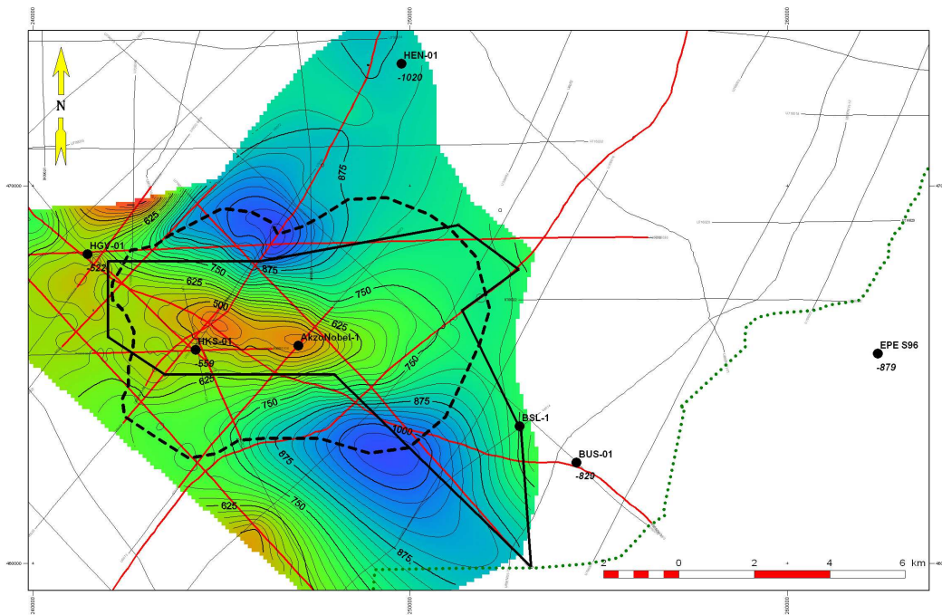
Figure 4.3 Depth map top Zechstein with drainage area. Within the drainage area the source rock of the Platten- and Hauptdolomit is not mature. Consequently no estimate of expelled hydrocarbons has been derived.
