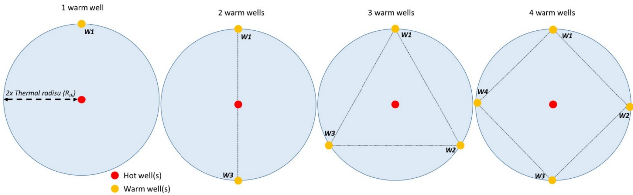
Figure 14. Placement rules for HT-ATES wells. An individual dot in these scenarios can consist of multiple clustered wells of the same type.
