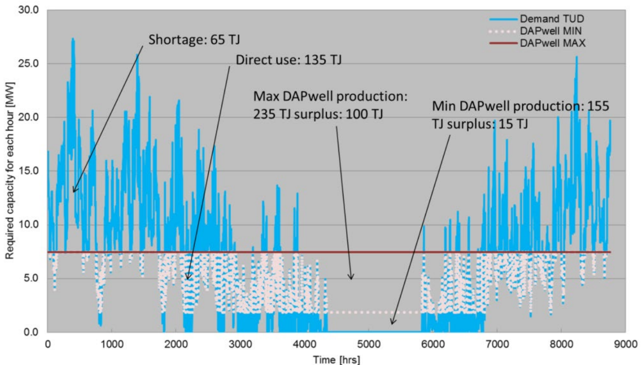
Figure 6: Heat demand campus and maximum potential geothermal production (rounded numbers).
