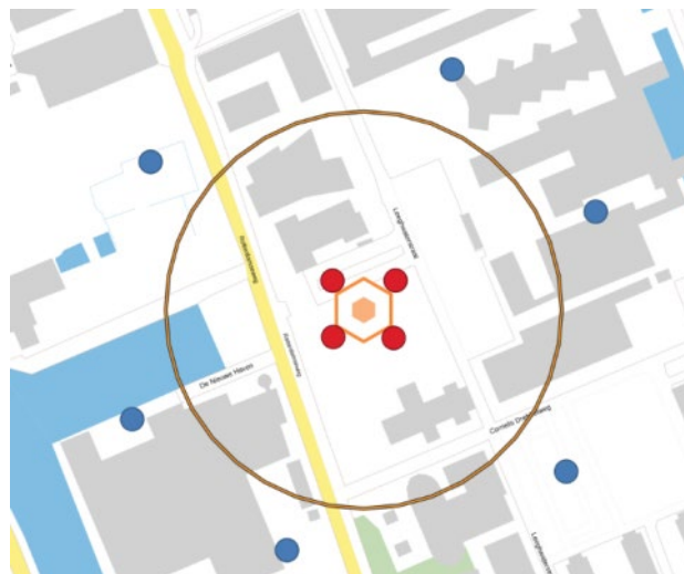
Figure 16. Sketch of possible HT-ATES system for the Ommelanden formation (10 total wells) locations in immediate area of DAPwell. Red and blue dots are hot and cold wells, respectively, brown circle is the maximum thermal zone.
