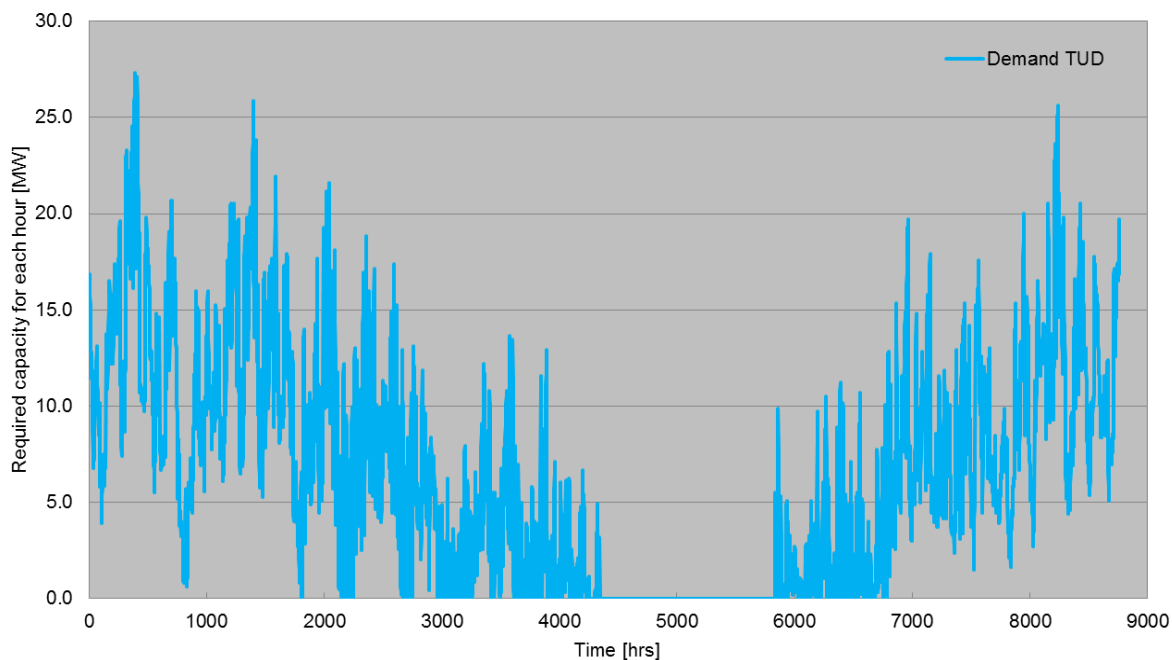
Figure 4: Current demand profile of the TU Delft campus (excluding the planned track 5).
