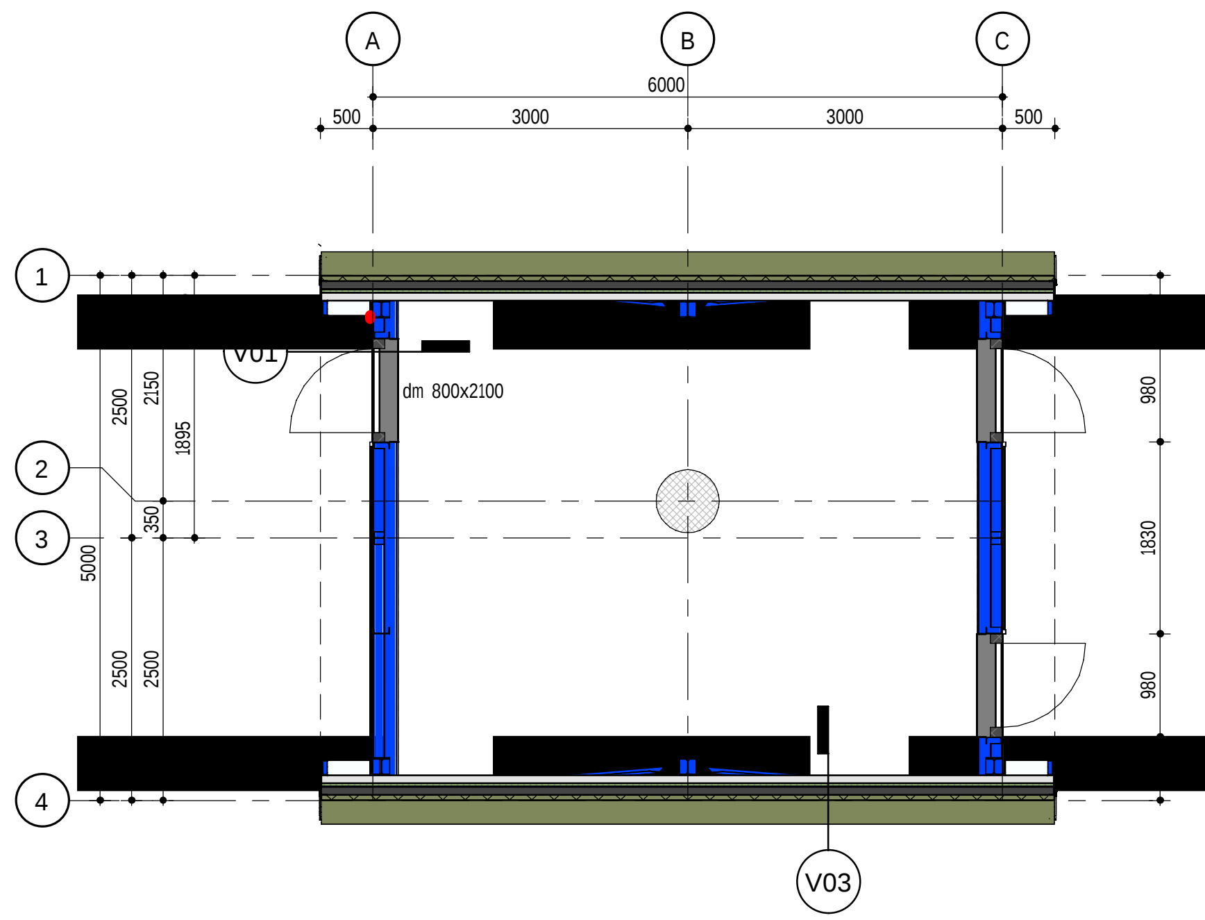
GROUND FLOOR, +2000 P 1 : 50
