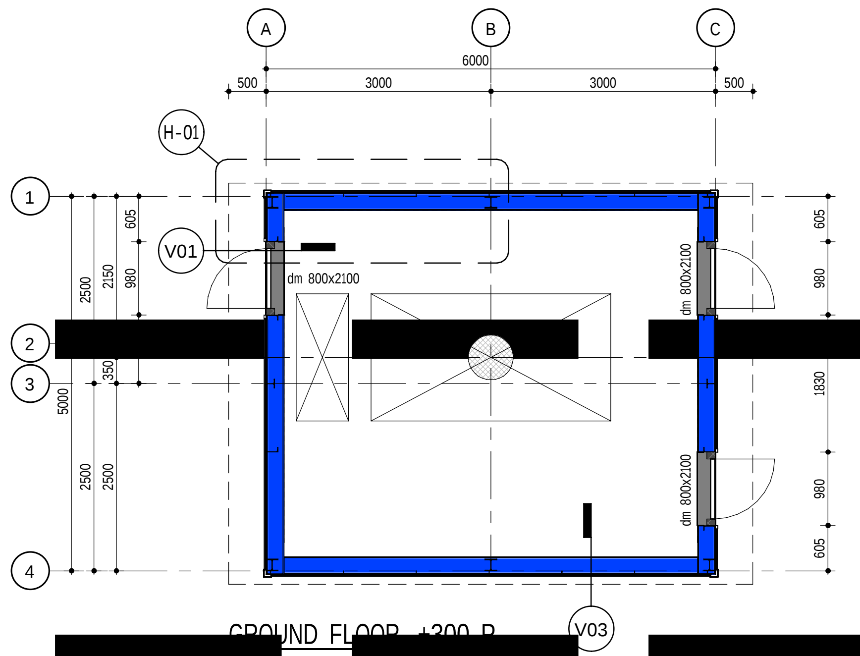
GROUND FLOOR, +200 P
