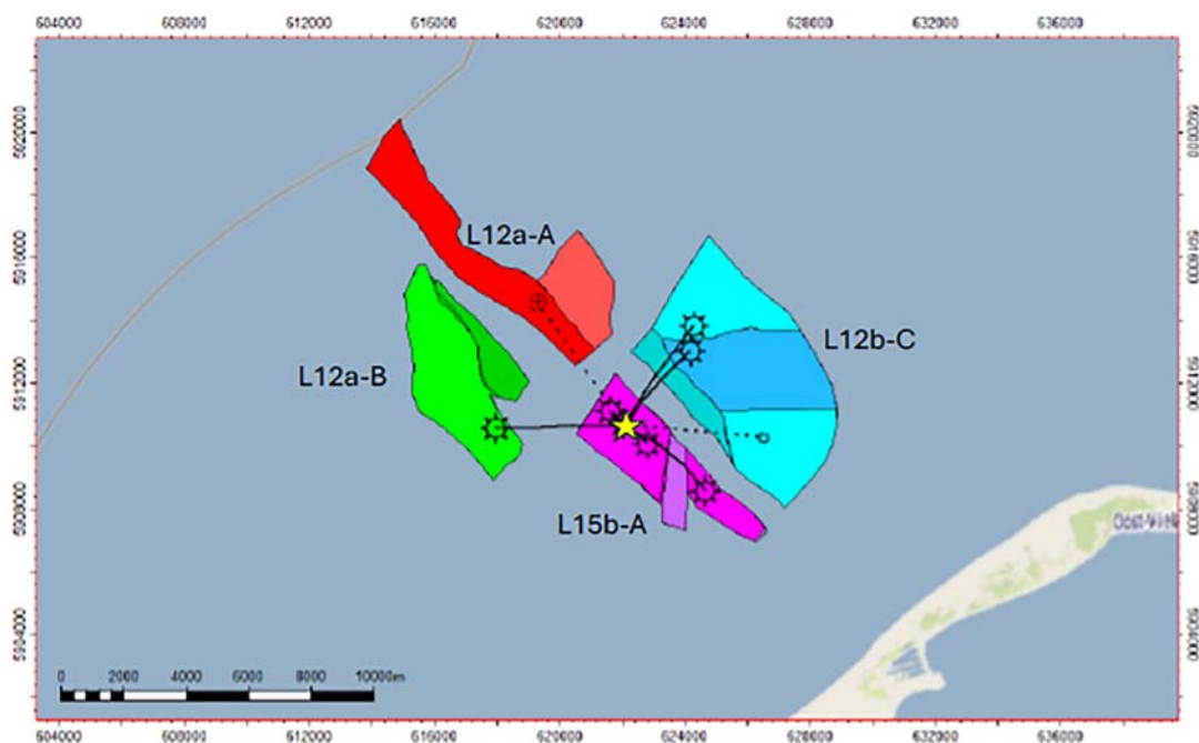
Locaties gasvelden winningsplan L12/L15 (bron: Eni)
