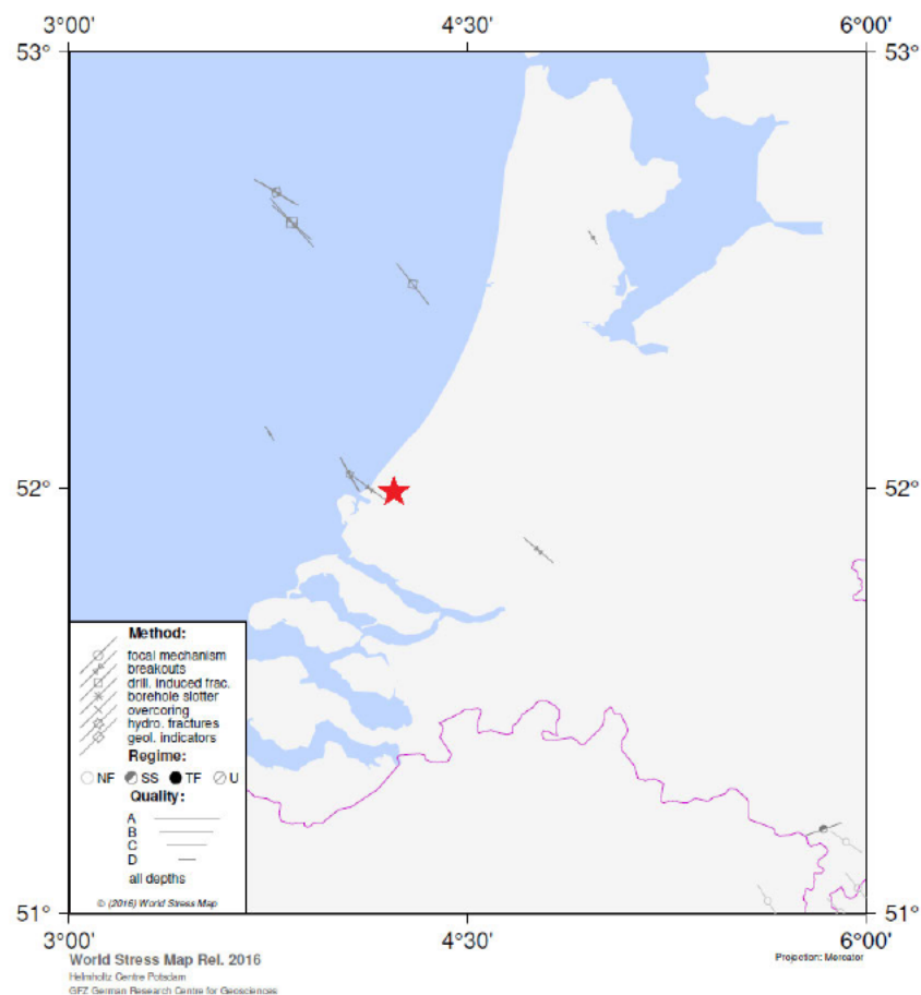
Figure 9: Map of stress field orientations for The Netherlands based on the World Stress Map [46]. Figure was generated using the onlinetool “CASMO” ( http://www.world-stress-map.org/casmo ). Project location is indicated by a red star.
