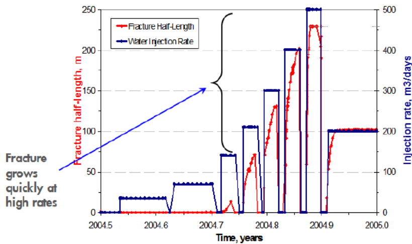
Figure 5: Injection scheme during 5-spot trial plus computed fracture lengths
