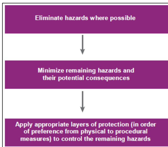
Figure 7 ALARP principle
