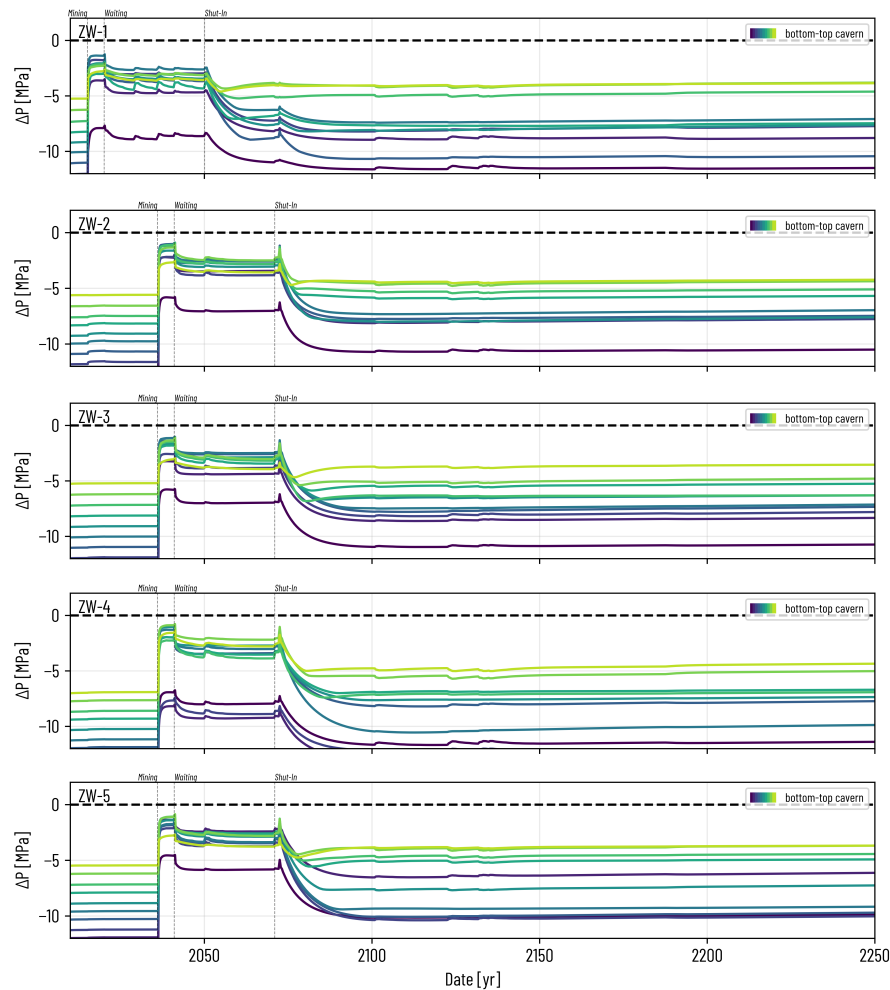
Fig. A120: Simulation I. Maximum dP over time, 25 m offset from cavern wall. Colors indicate different evaluation heights.
