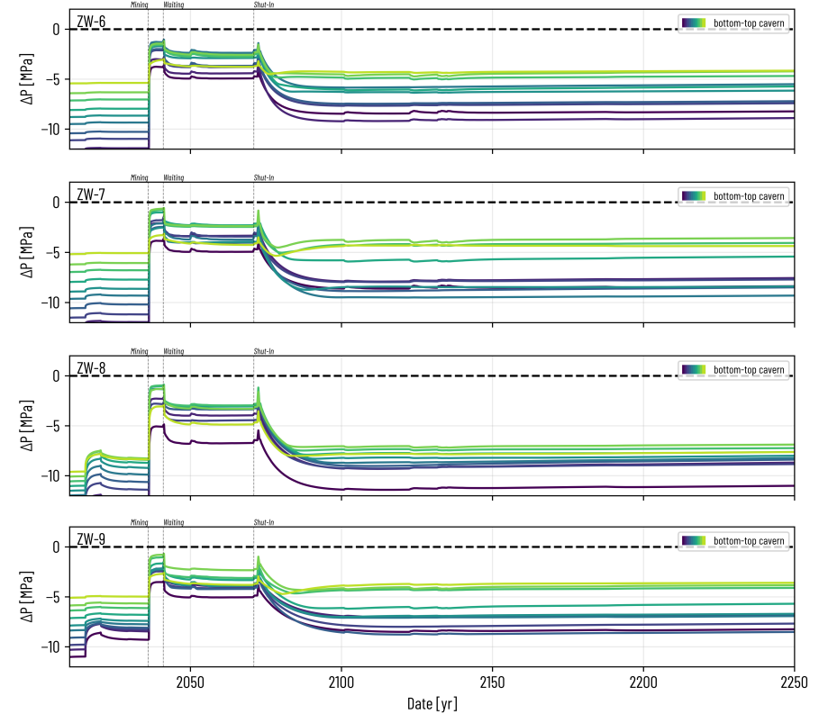
Fig. A120: Simulation I. Maximum dP over time, 25 m offset from cavern wall. Colors indicate different evaluation heights.
