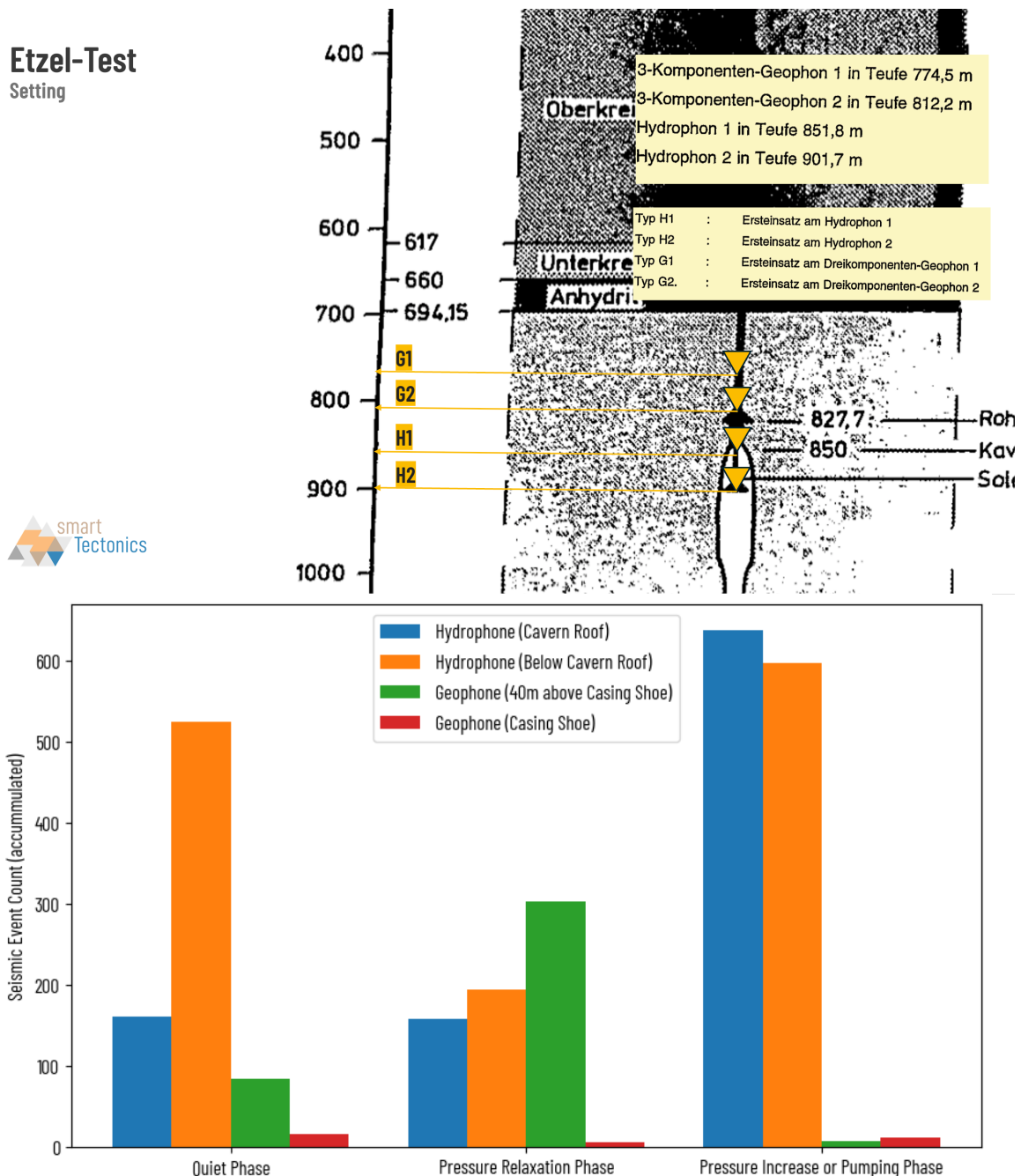
Figure 14 Top: Configuration of geophones and hydrophones used for seismic monitoring during the Etzel test (modified from Denzau et al, 1994). Bottom: Distribution of occurring acoustic and microseismic events during the Etzel test.
